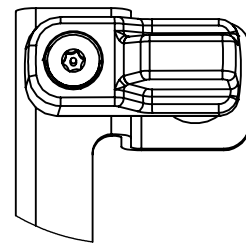
DETAIL B (CLOSED) SCALE 1 : 1.5
